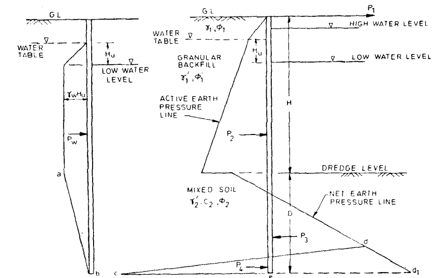
6A Distribution of Unbalanced Water Pressure
